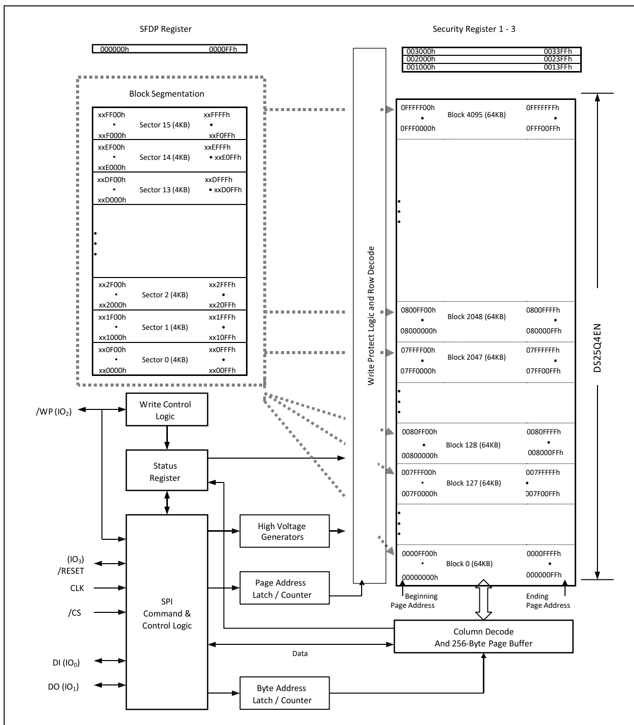
Figure 2. DS25Q4EN Serial Flash Memory Block Diagram
